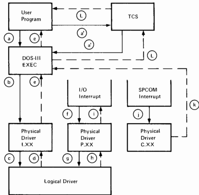
Figure 2. Processing I/O Requests
